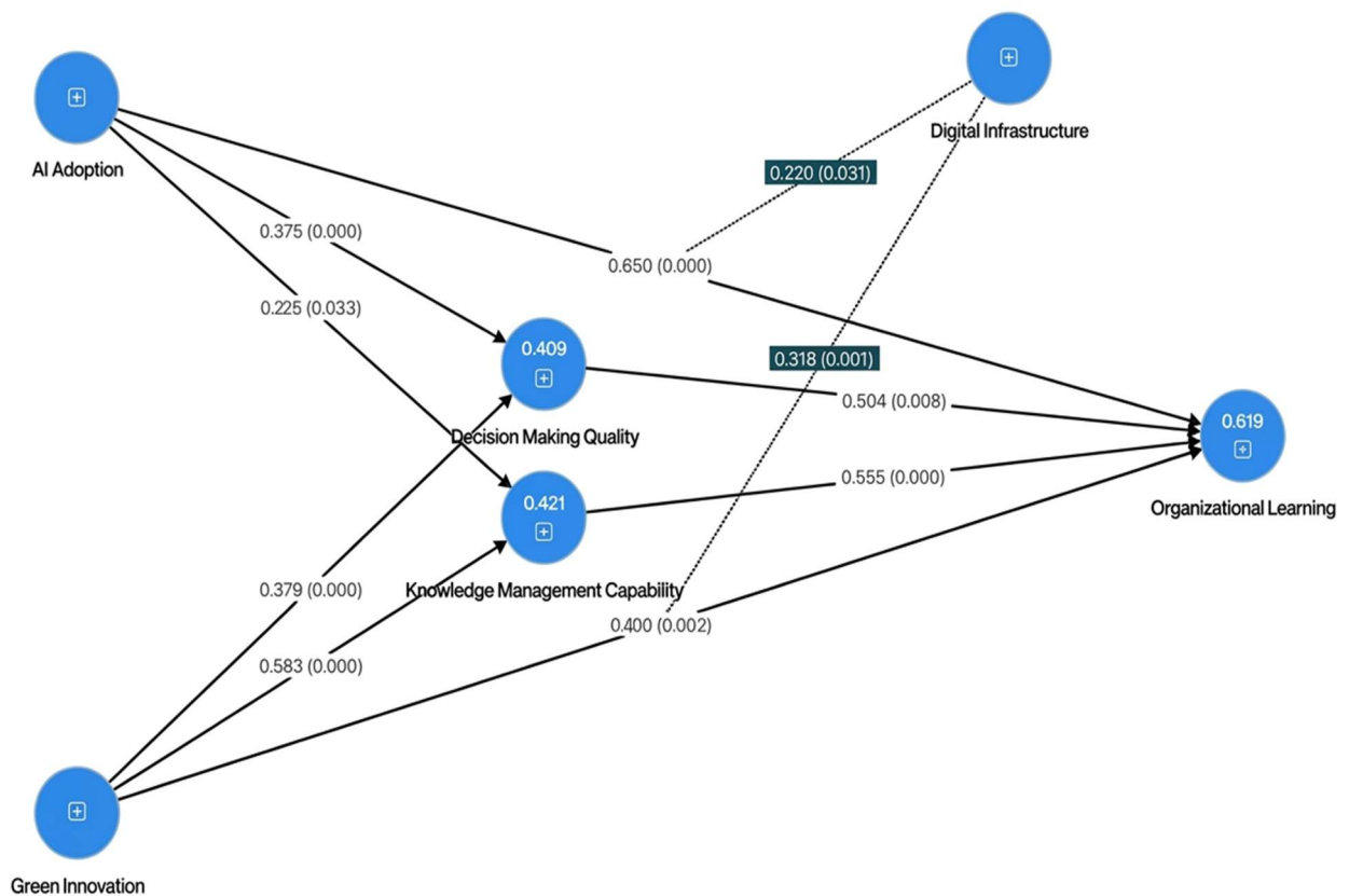
Figure 2. PLS-SEM Structural model.
